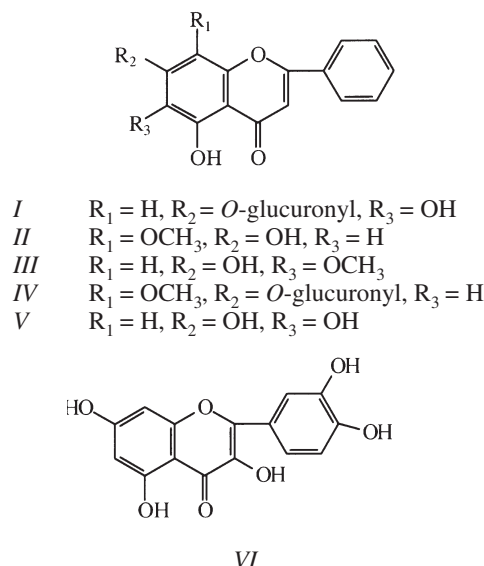
Fig. 1. The structural formulae of flavonoids used in this study
