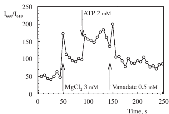
Fig. 1. Measurement of \Delta\psi in reconstituted yeast ( S. pombe ) plasma membrane proteoliposomes by the fluorescent probe Oxonol VI
